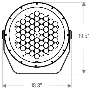
Standard Bracket
