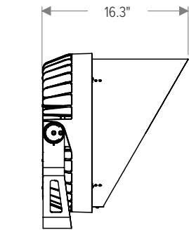
With Visor (JSPRMK2-VISOR)
